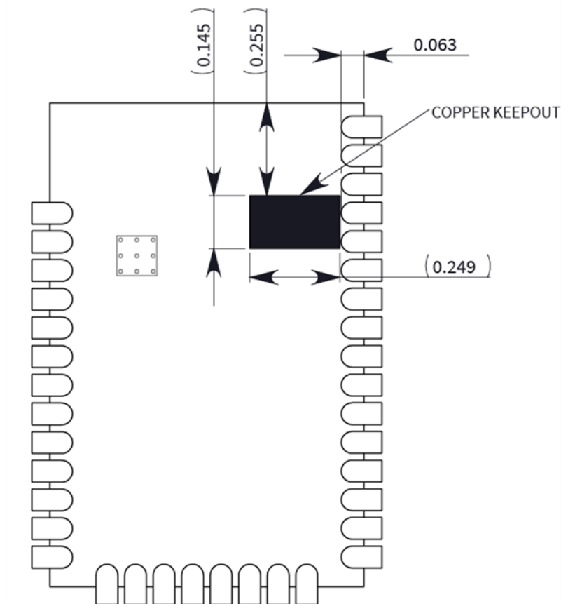
SMT footprint showing required copper keepout (all layers)
